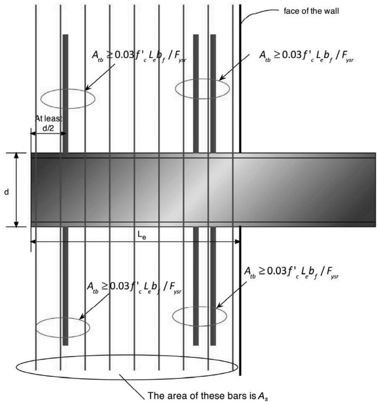
Fig. C-H5.2. Transfer bars.
