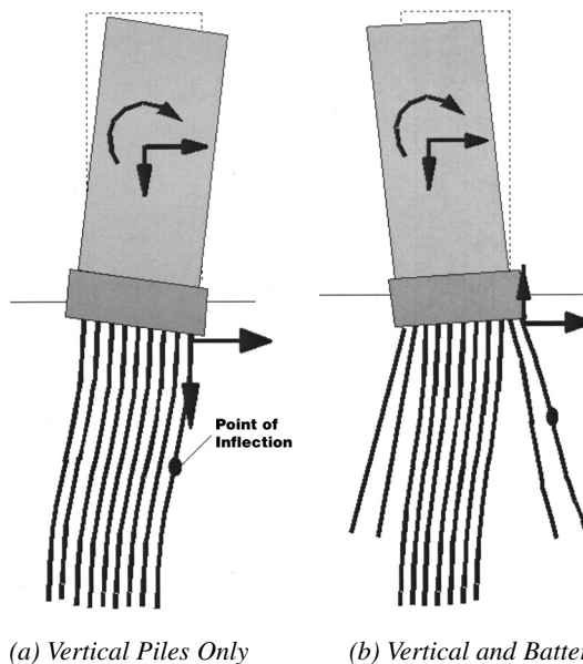
Fig. C-D4.1. Deformations of piles and forces acting on an individual pile.
