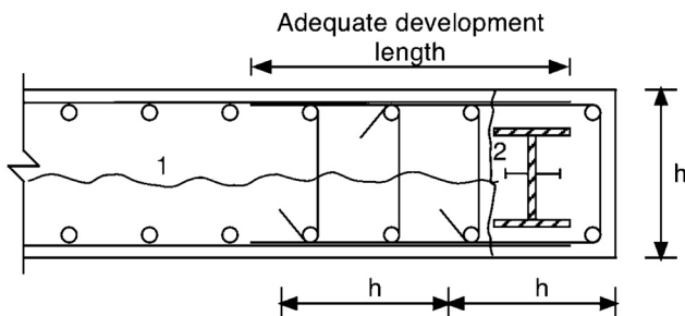
Fig. C-H5.1. Reinforcement to prevent splitting failures.
