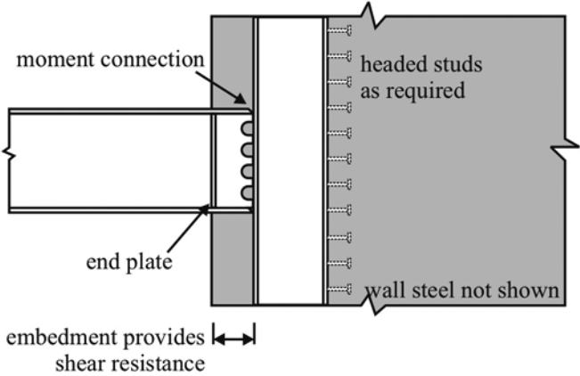
(a) Steel coupling beam attached to steel wall boundary element column
