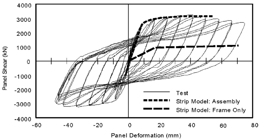
Fig. C-F5.6. Comparison of experimental results for lower panel of multi-story SPSW frame and strength predicted by strip model (after Driver et al., 1997).
