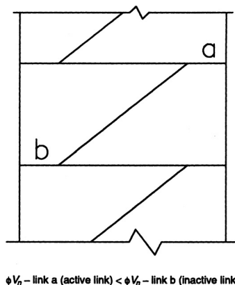
Fig. C-F3.2. EBF—active and inactive links.
