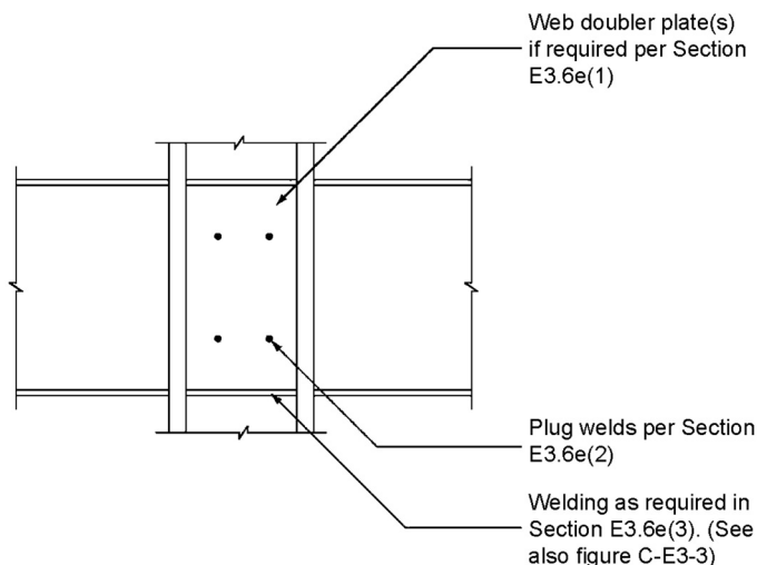
Fig. C-E3.2. Connecting web doubler plates with plug welds.
