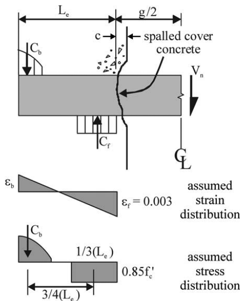
Fig. C-H4.6. Method for computing the embedment capacity.
