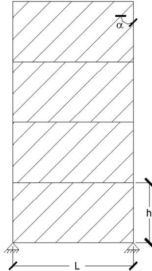
Fig. C-F5.5. Strip model of an SPSW.
